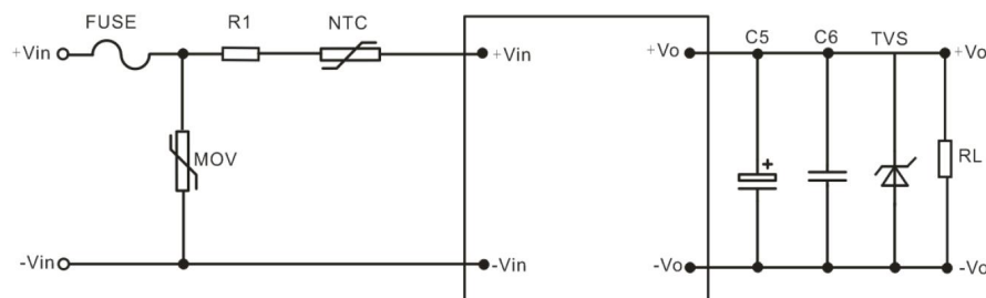
Figure – Circuit 1
