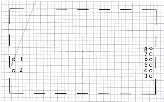
PCB layout vertical view Grid 2.54x2.54[0.10x0.10]
