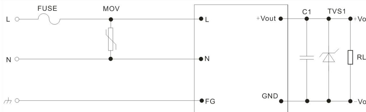
Recommended circuit 1
