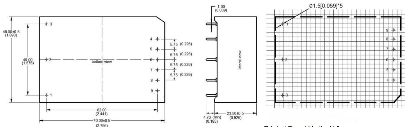
Printed Board Vertical View
