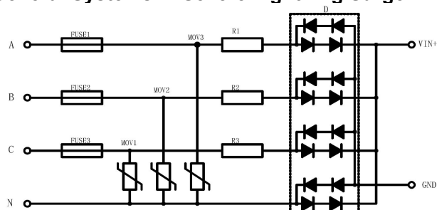
Figure 3: Recommended External Circuit for 4 kV Differential-Mode Surge with High Requirements - Full-Wave Rectification
