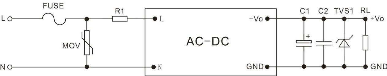
Figure – Circuit 1
