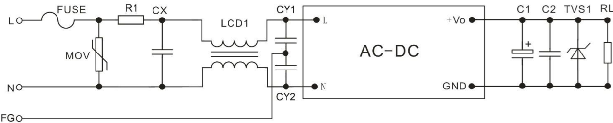
Figure – Circuit 2
