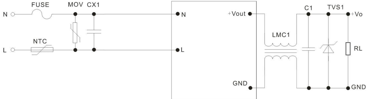
Recommended Circuit 1
