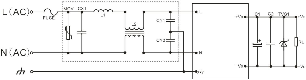
Circuit 1: Recommend circuits for higher EMC requirements
