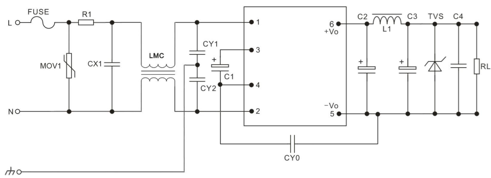
Figure - Circuit 2-3
