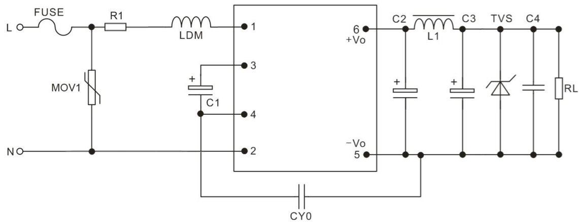
Figure - Circuit 2-4
