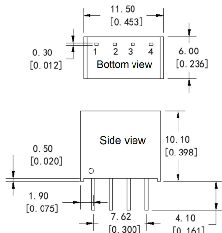
Mechanical Outline Drawing
