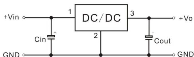
Positive output application circuit
