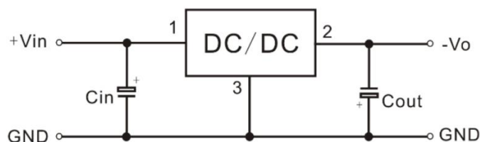
Negative output application circuit
