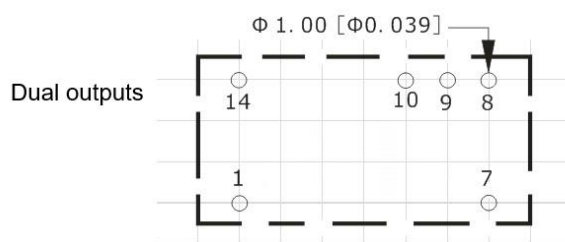
PCB layout vertical view
